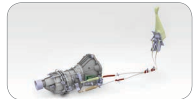
Cable operated gear shifts for Car-like driving
